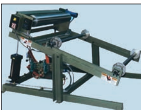
Roll Stand / Payout with Auto Roll Load
